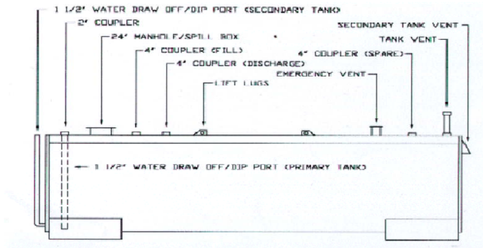
Dimensional Chart
