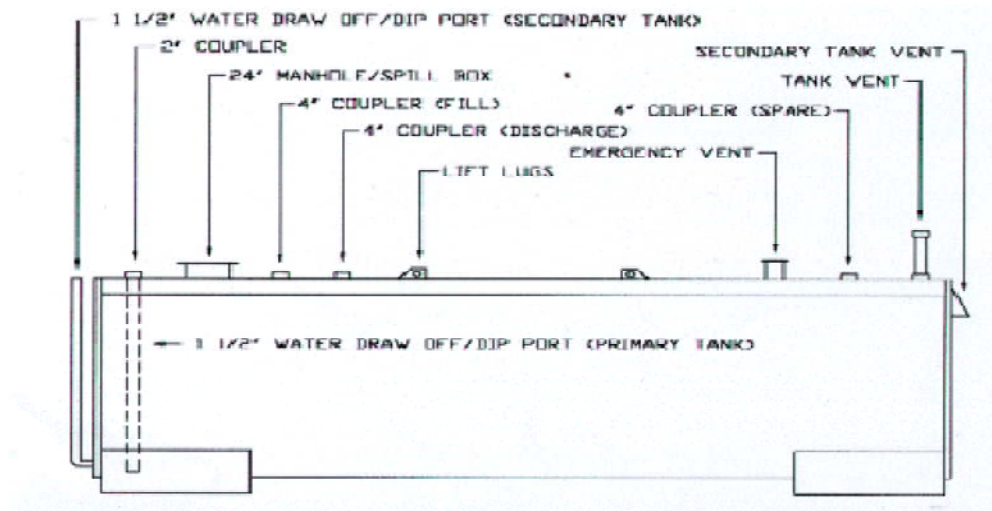
Dimensional Chart
